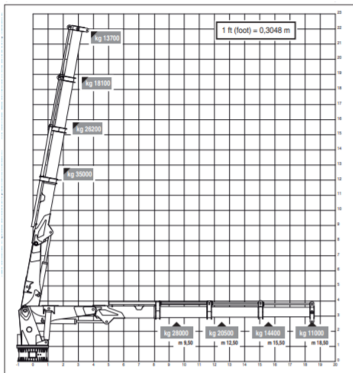
Foreship crane : Heila HLRM 280-3SL
