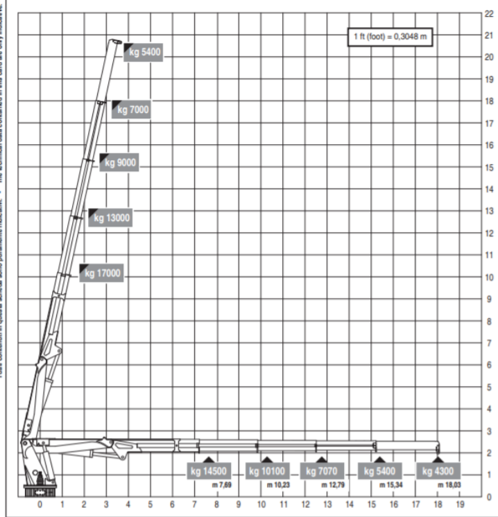
Aftship crane : Heila HLRM 120-4SL
